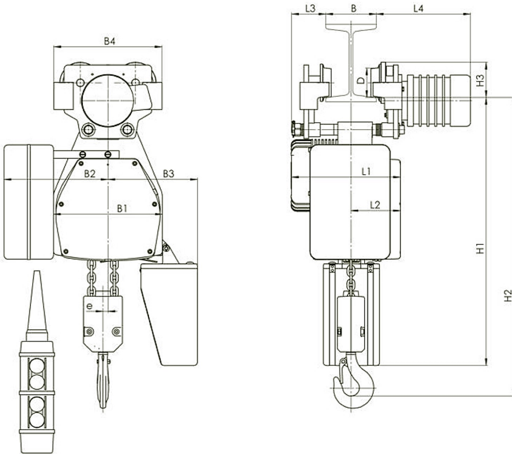
Chain electric hoist type BE, driven by a motor cart
